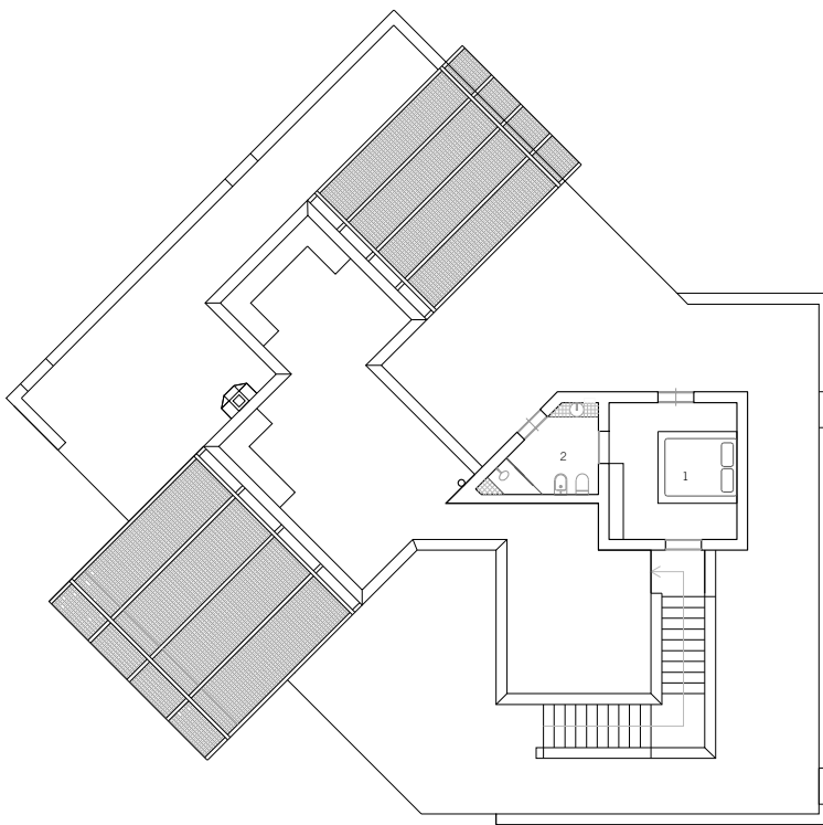
pianta piano primo/ first floor plan
