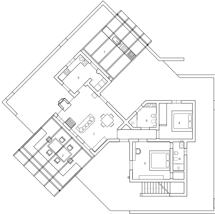
pianta piano terra/ ground floor plan
